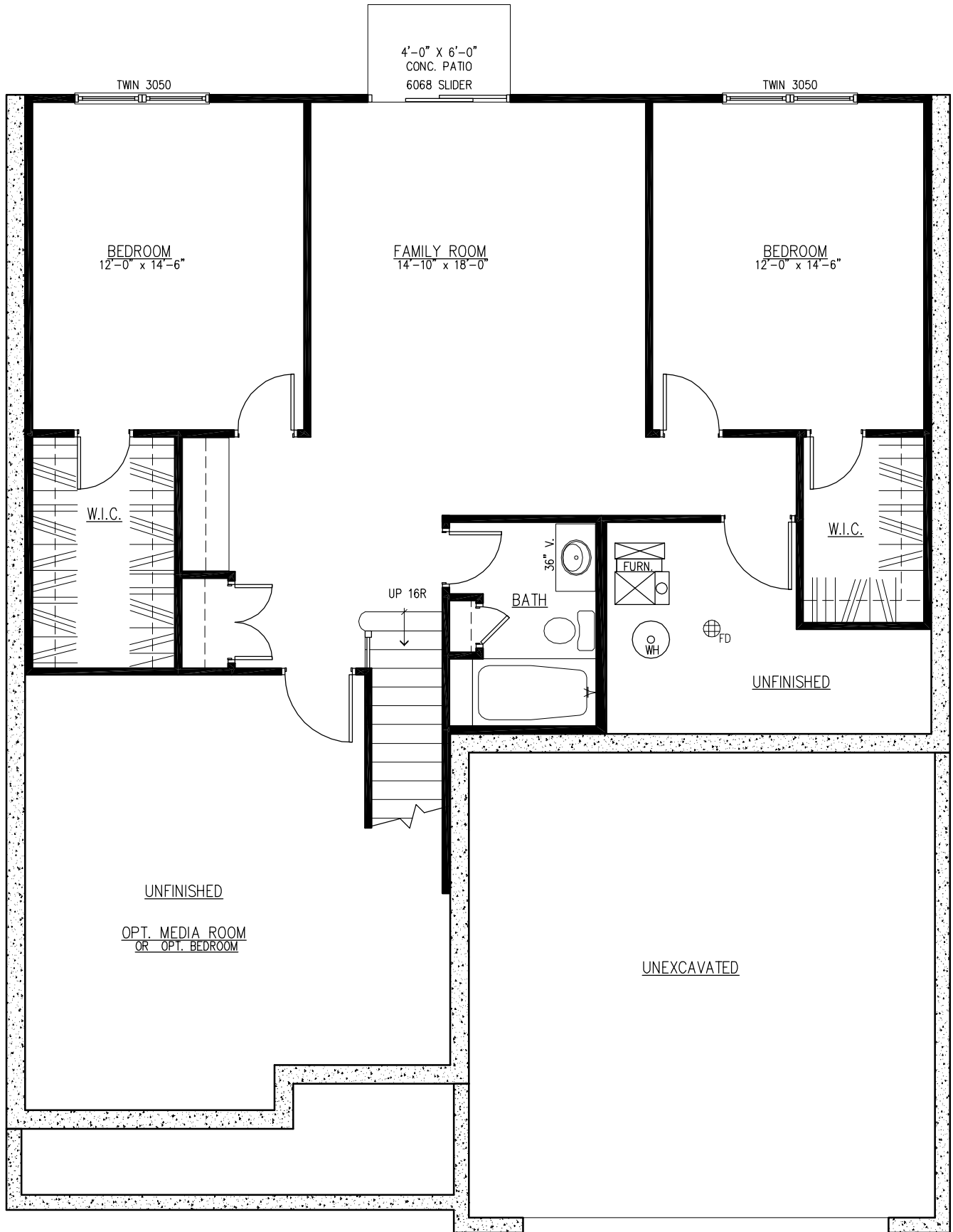
FINISHED BASEMENT 985 SQ. FT.
